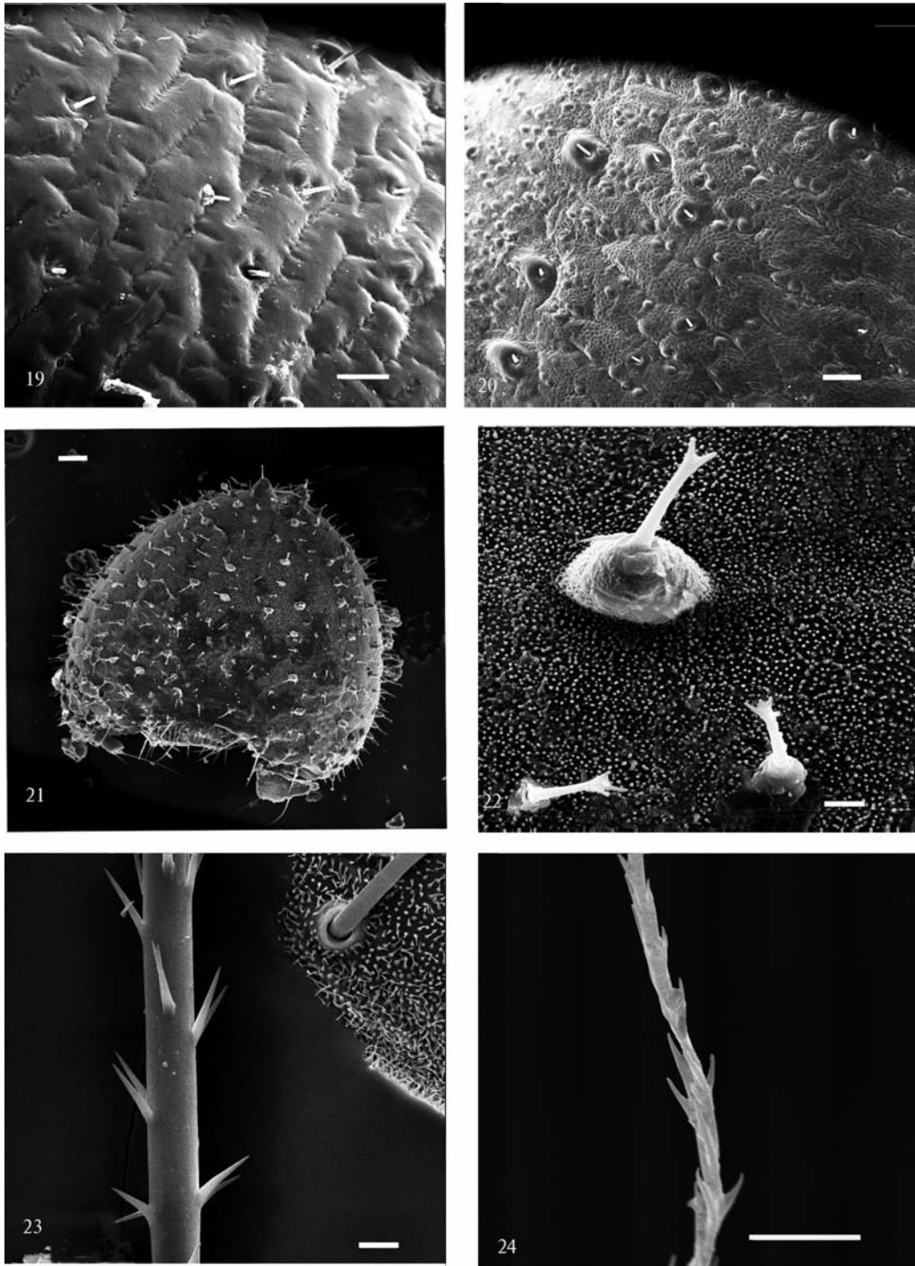
Fig. 19–24. Larval head: 19–22 — Sphingidae; 23–24 — Erebidae: Lymantrinae; 19 — head capsule of 5th instar Agrius convolvuli ; 20 — head capsule of 5th instar Smerinthus planus ; 21 — head capsule of 2nd instar Smerinthus planus ; 22 — setae of 2nd instar Smerinthus planus ; 23 — plumose setae of 4th instar Teia dubia ; 24 — plumose setae of 2nd instar Arctornis l-nigrum . Scale bars: 19–21 — 100 \mu ; 22–24 — 10 \mu .
