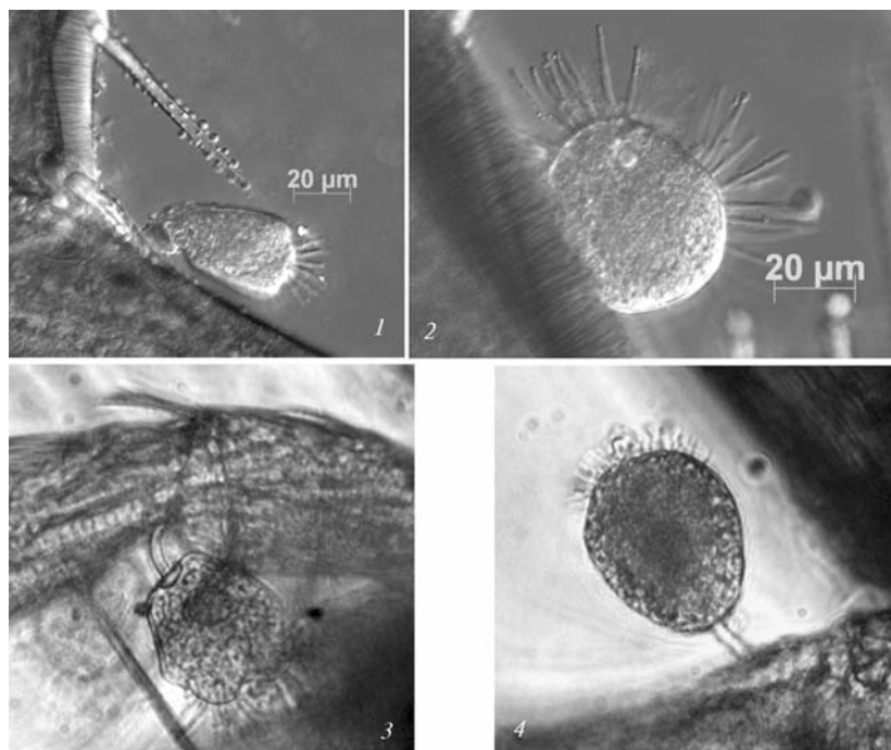
Fig. 2. Tokophrya wenzeli : 1–2 — from Ukrainian water bodies (differential interference contrast; 1 — lateral view, 2 — frontal view); 3 — from Poland (x640); 4 — from Lake Ohrid (Macedonia) (x640).
