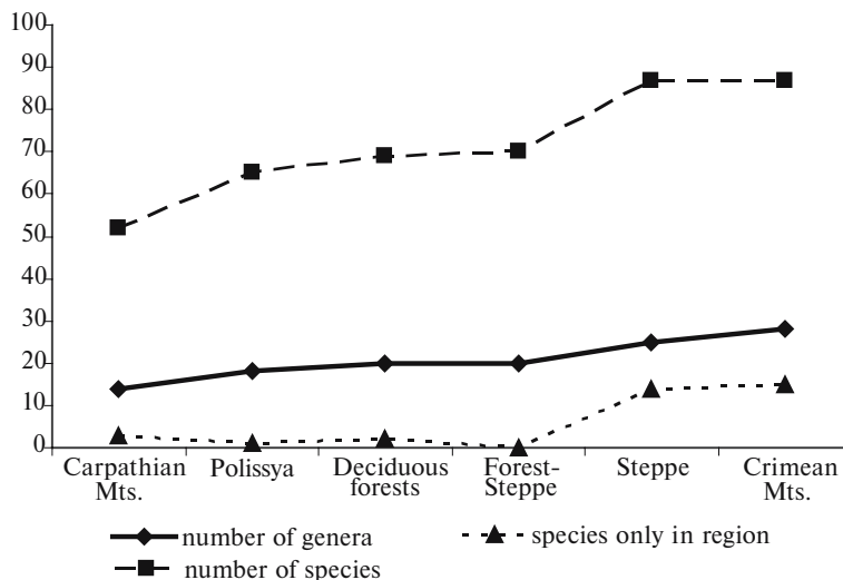
Fig. 1. Number of species and genera of ants in different natural zones of Ukraine.
